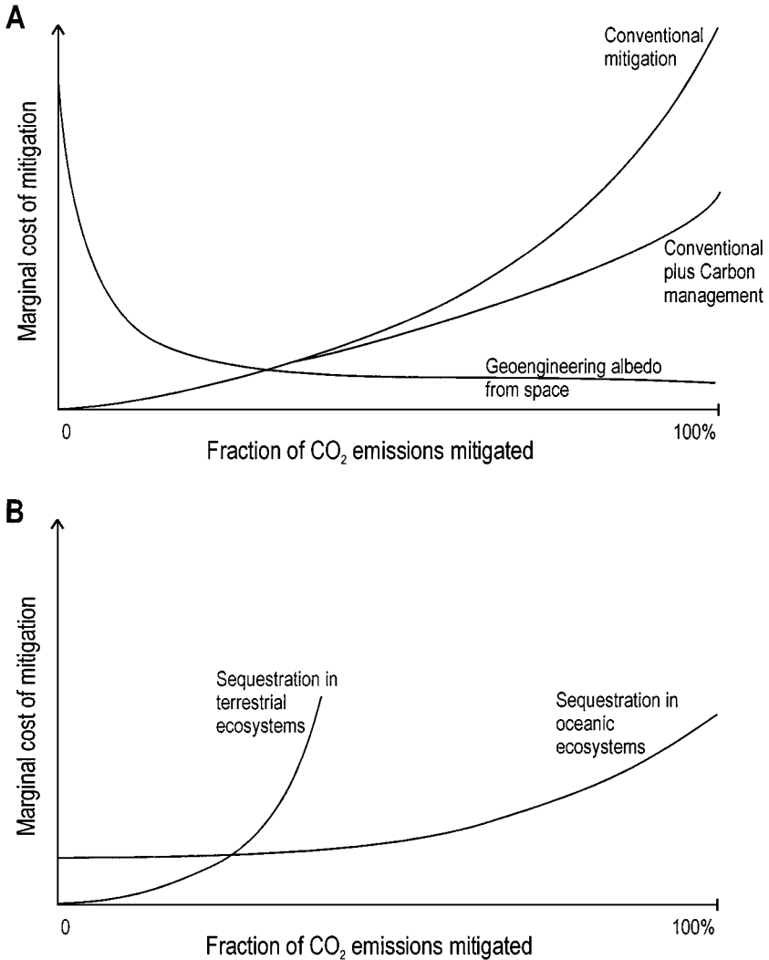
Figure 4 Schematic comparison between modes of mitigation. (A) Conventional mitigation means any method other than geoengineering or carbon management, e.g. conservation or use of nonfossil energy. The addition of carbon management lowers the cost of emissions mitigation; however, costs will still rise steeply as one tries to eliminate all emissions. Conversely, albedo modification from space has very high initial capital costs but can provide essentially unlimited-effect low marginal cost. (B) Sequestration based on ecosystem modification will have costs that rise steeply at a mitigation amount (carbon flux) set by the internal dynamics of the respective systems.
