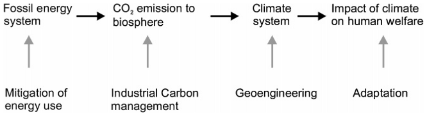
Figure 2 Four-part schema of the climate problem. The interpretation follows that of Figure 1. Note the distinction between mitigation of fossil energy use, carbon management, and geoengineering that illustrate the definition described in Section 2.
