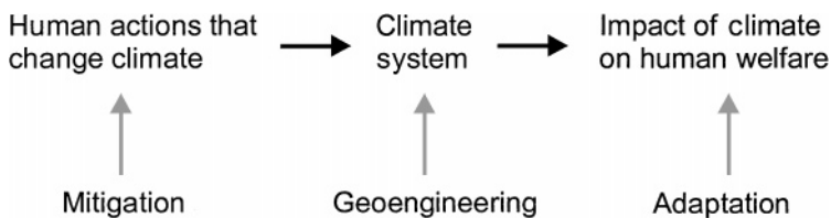
Figure 1 Three-part schema of the climate problem. The horizontal arrows in the top row show the causal chain in this version of the anthropogenic climate problem. The vertical arrows and the bottom row define the modes of intervention.
